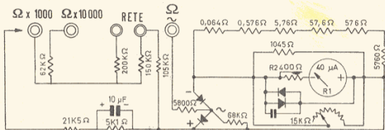
Schema Ohmetro in C.A.
